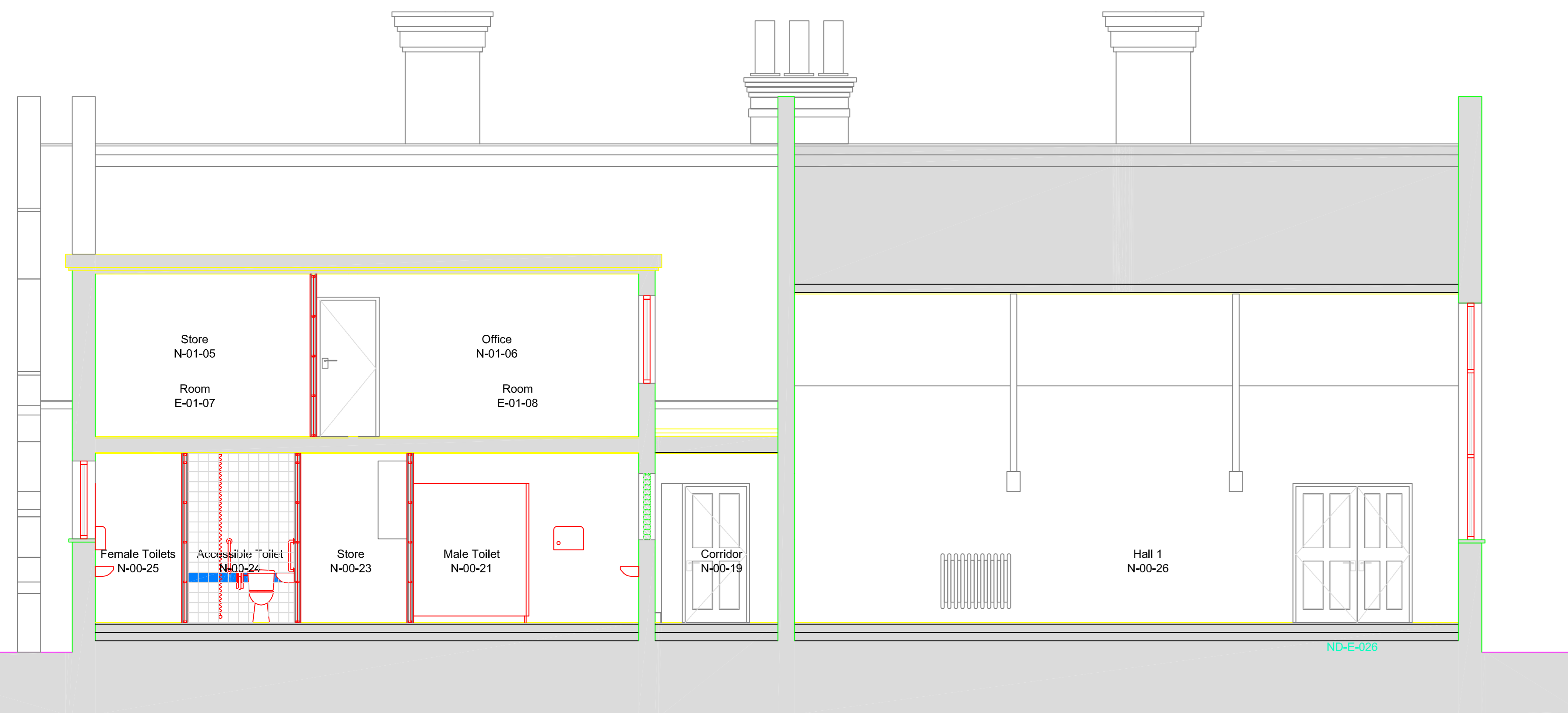
Section H-H Scale 1/50
