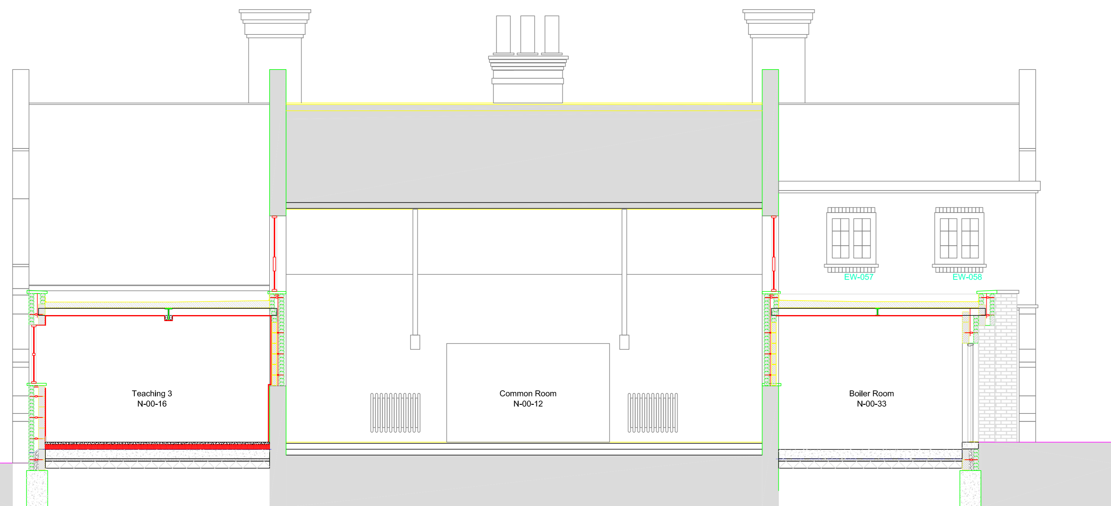
Section M-M Scale 1/50
