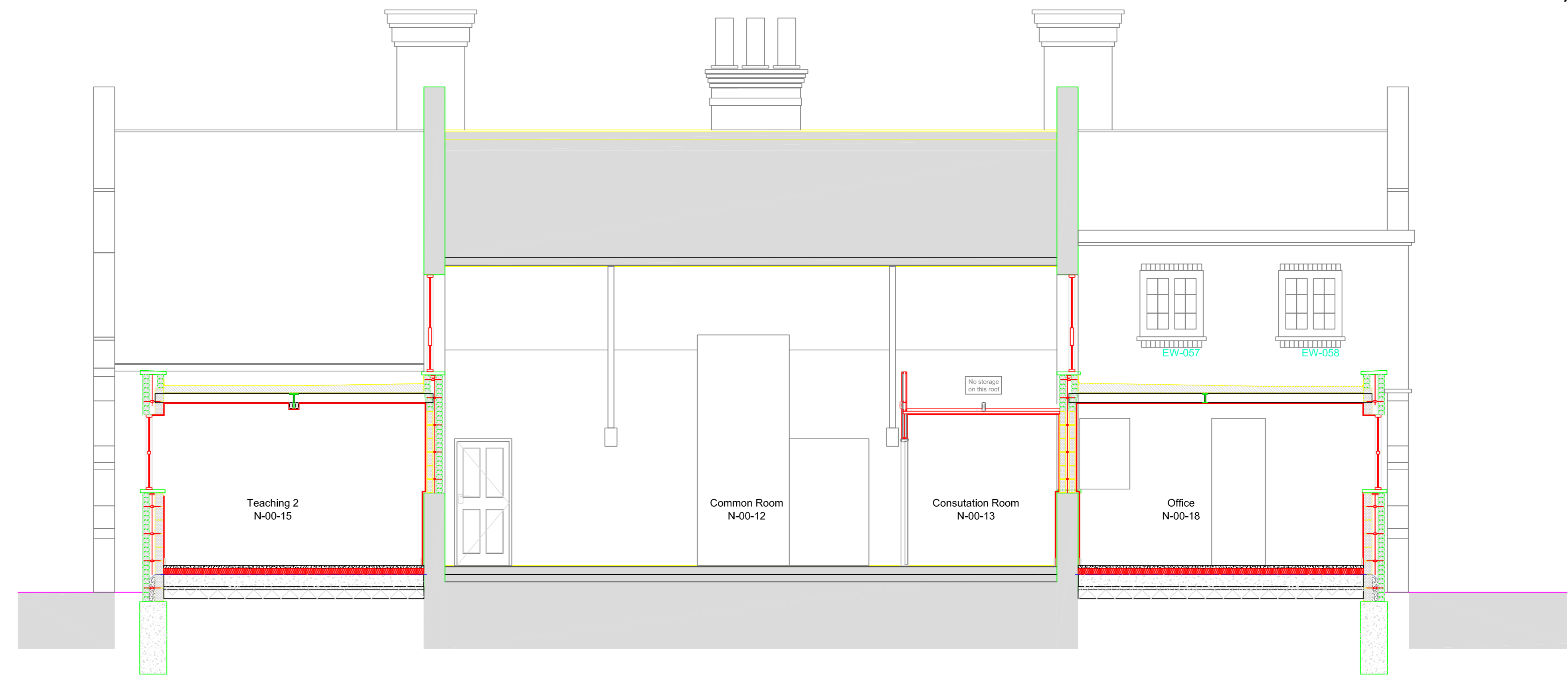
Section P-P Scale 1/50
