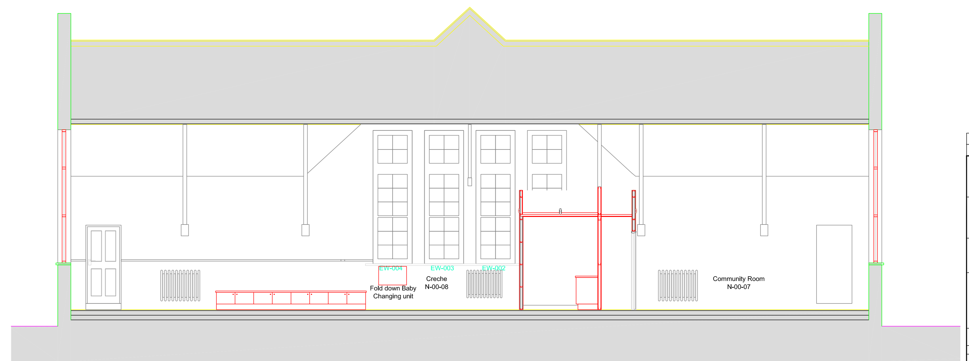
Section T-T Scale 1/50
