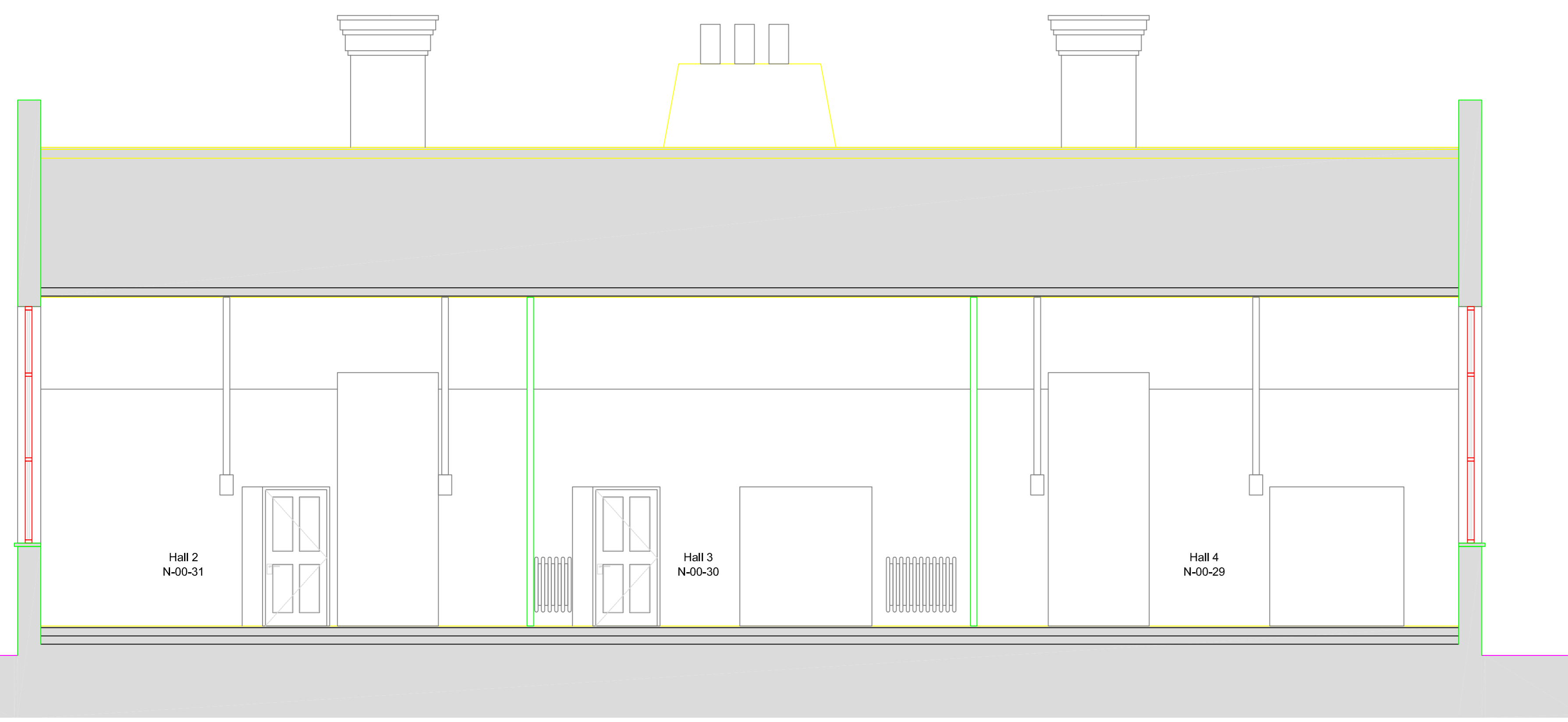
Section H-H Scale 1/50
