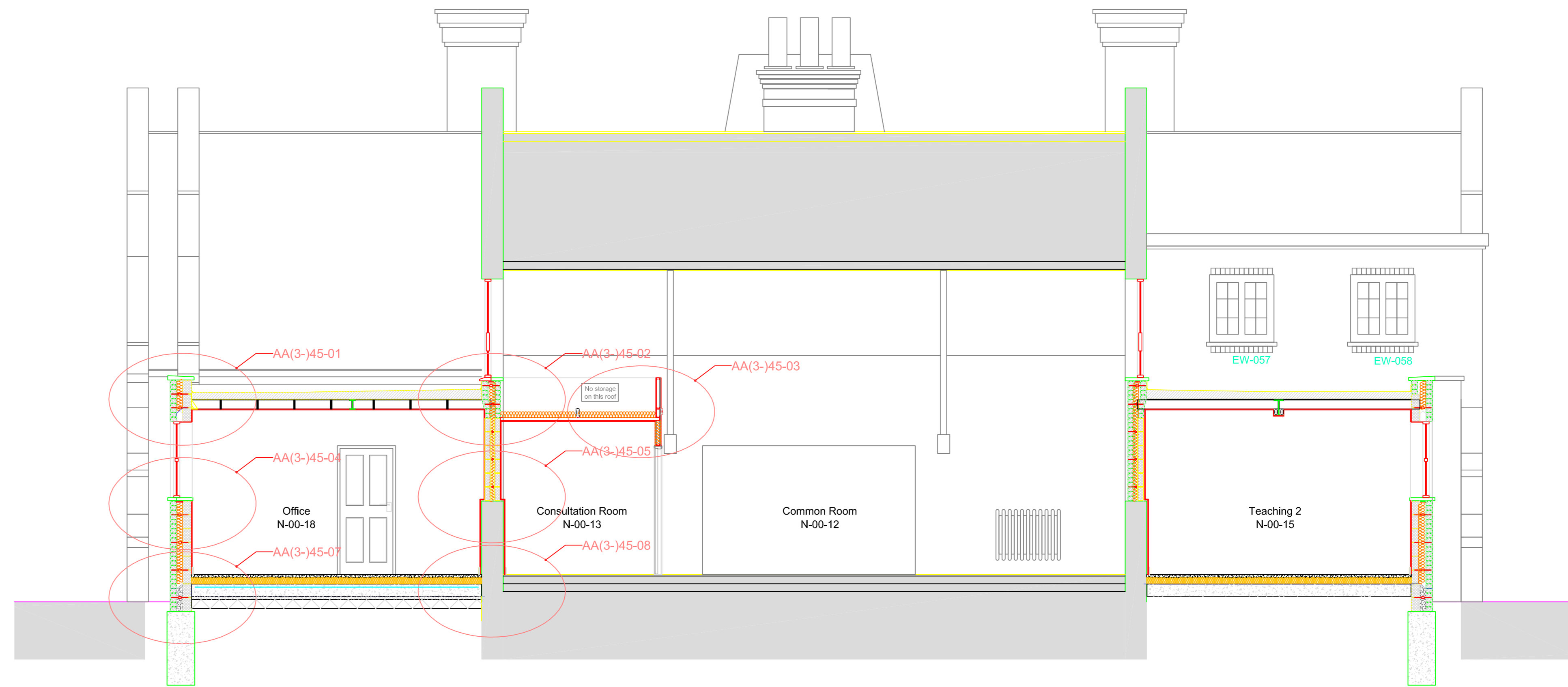
Section N-N Scale 1:50
