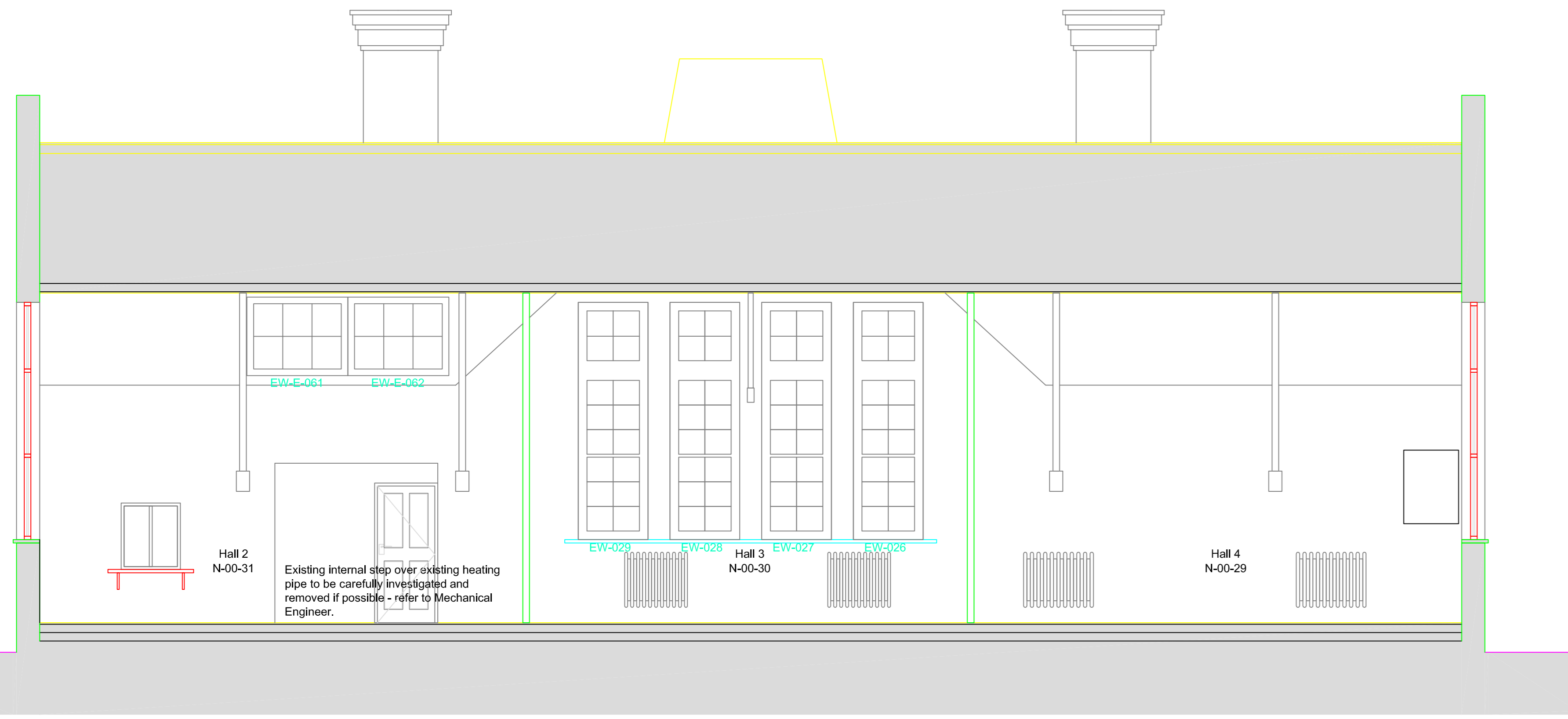
Section G-G Scale 1:50
