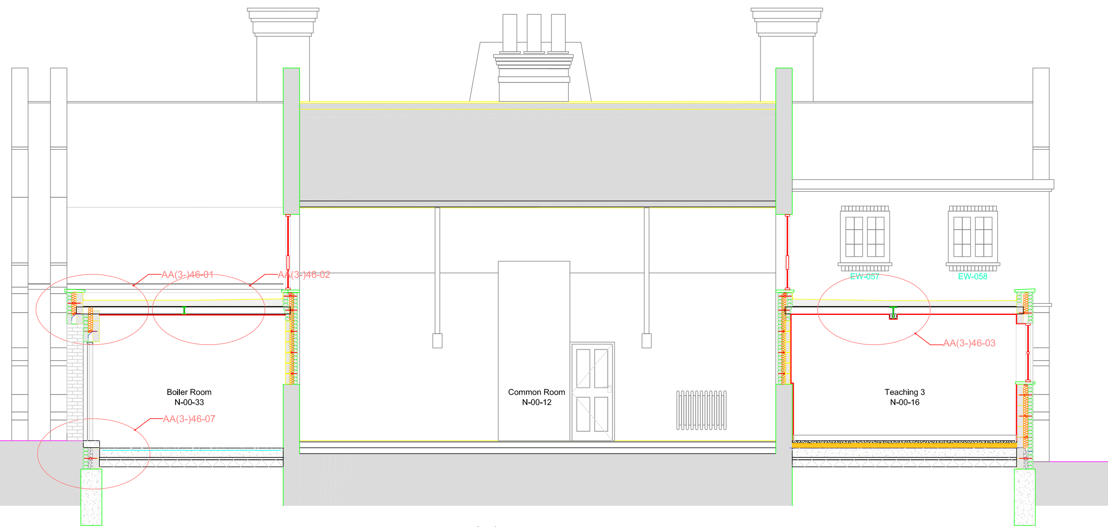
Section L-L Scale 1:50
