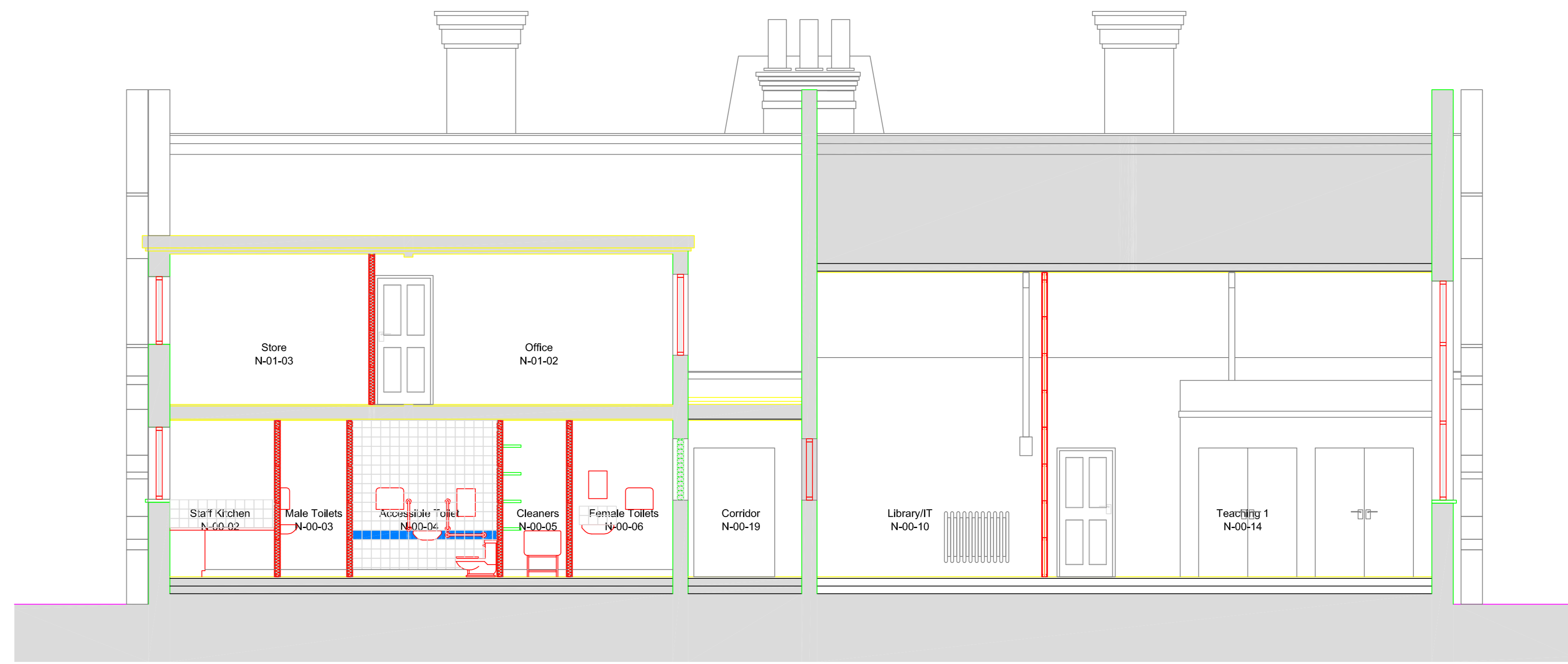
Section Q-Q Scale 1:50
